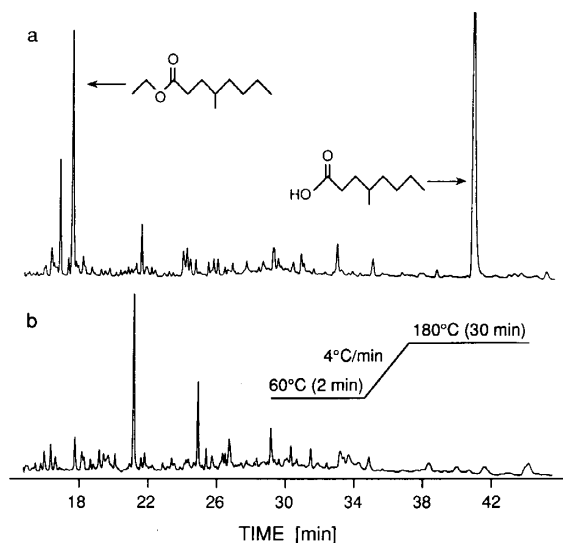
Fig. 1. Gas chromatograms of volatiles from male ( n = 13 ) (a) and female ( n = 11 ) (b) O. monoceros maintained in aeration chambers for 168 h without provision of food. Chromatography: Hewlett-Packard 5830 A equipped with a glass capillary column (30 m×0.5 mm ID) coated with SP-1000.
